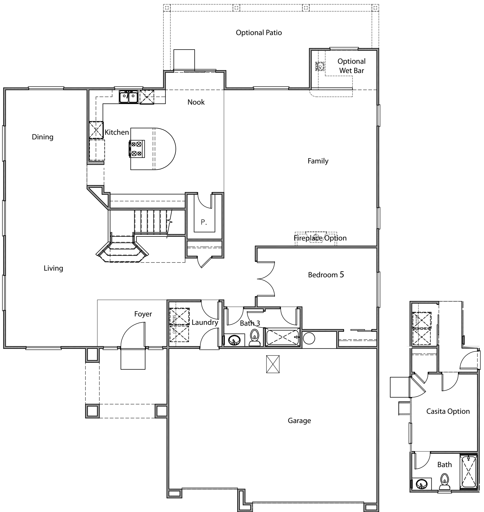
Rivendell Plan 4035-1st Floor
